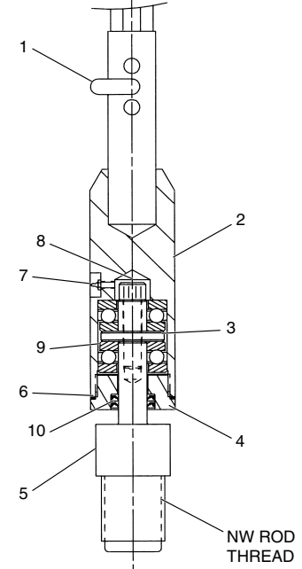
Bearing Assembly
