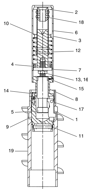
Latch Assembly
