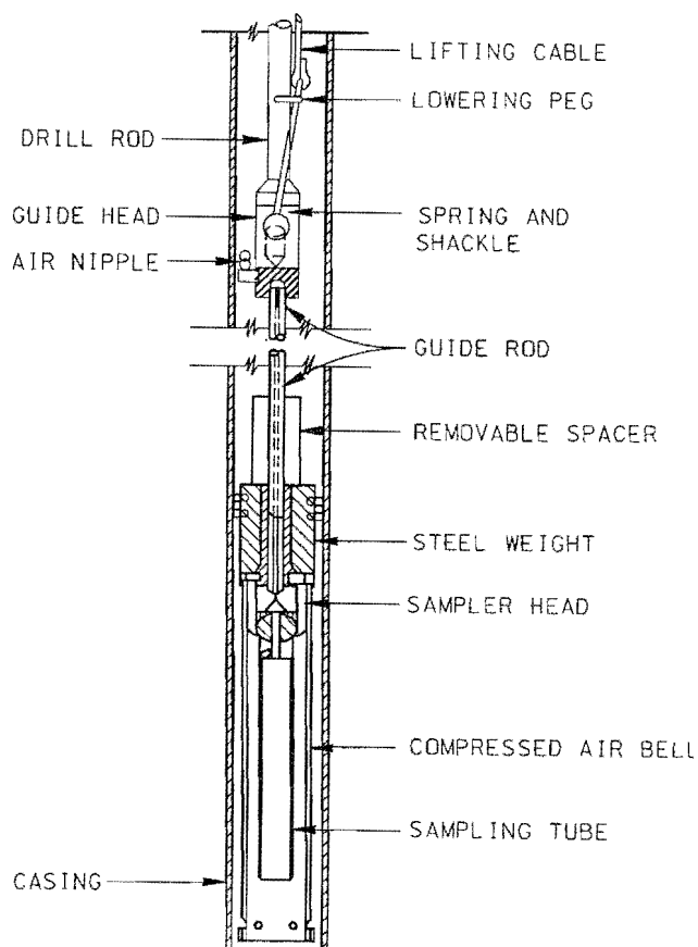
FIGURE 5-18. Bishop Sand Sampler (after Hvorslev 1949)
